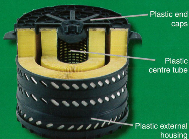
Design of MANN+HUMMEL filter
