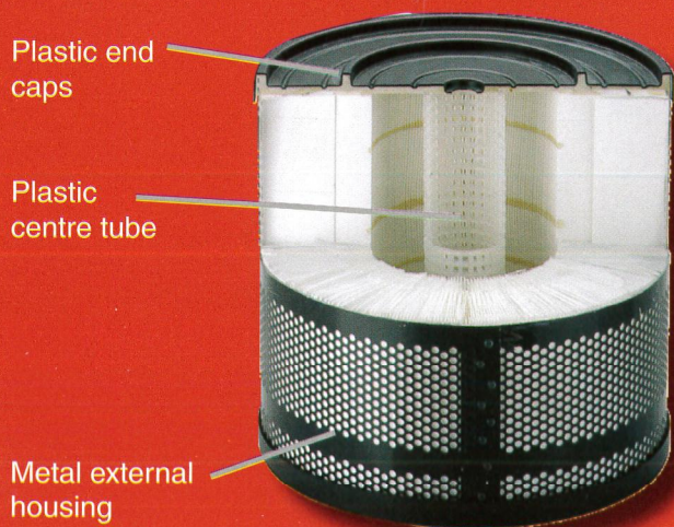
Design of hybrid filter
