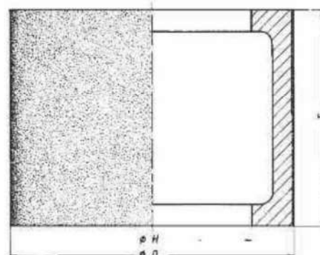
TYPE 47 - Centerless-Schleifscheiben, mehrlagig Centerless-grinding wheels, multilayer
